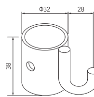
HANGER U-TYPE, U형거
