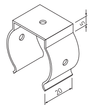
BOARD FIXING-B, 판지고정금구-B
