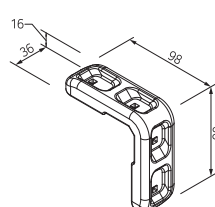
RIGHT ANGLE BUMPER
