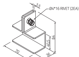
PANEL GUIDE (U TYPE)
