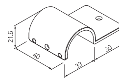
BOARD FIXING-A, 판지고정금구-A
