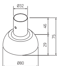
OVERLAP CAP 중복캡
