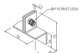
PANEL GUIDE (L TYPE)
